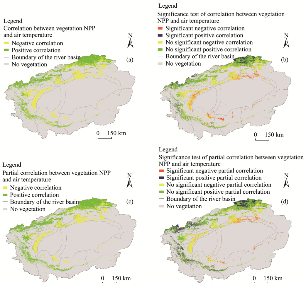
Fig. 8 Spatial distribution of the correlation (a), significance test of correlation (b), partial correlation (c), and significance test of partial correlation (d) between vegetation NPP and air temperature in the Tarim River Basin during 2001–2020
