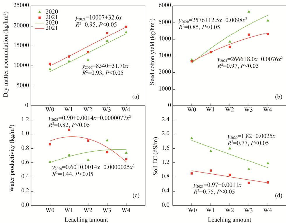
Fig. 9 Relationships of dry matter accumulation (a), seed cotton yield (b), water productivity (c), and soil EC (d) with leaching amount in 2020 and 2021
