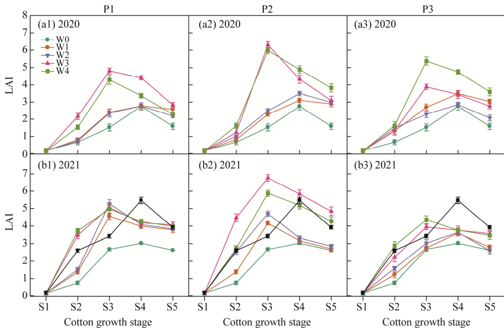
Fig. 8 Effects of different leaching amount and period treatments on leaf area index (LAI) of cotton in 2020 (a1–a3) and 2021 (b1–b3)
