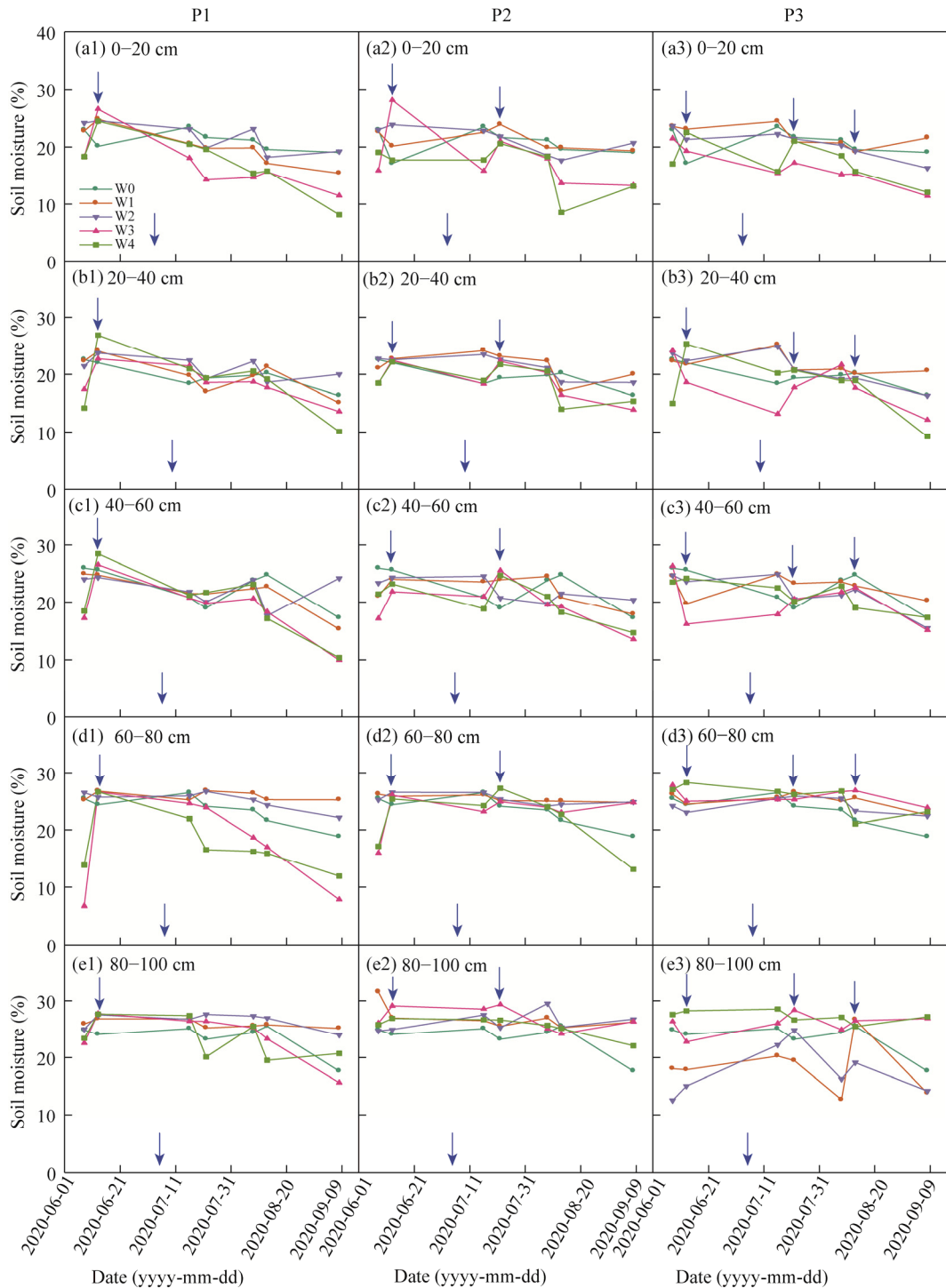
Fig. 3 Soil moisture dynamics for different leaching amount and period treatments in 2020. (a1–a3), 0–20 cm; (b1–b3), 20–40 cm; (c1–c3), 40–60 cm; (d1–d3), 60–80 cm; (e1–e3), 80–100 cm; W0, W1, W2, W3, and W4 represent leaching amount of 0.0, 75.0, 150.0, 225.0, and 300.0 mm, respectively. P1, seedling stage; P2, seedling and squaring stage; P3, seedling, squaring, and boll flowering stage. Arrow means the leaching date. The abbreviations of treatments are the same in the following figures and tables.
