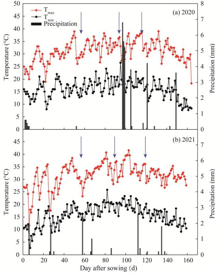
Fig. 1 Precipitation, maximum temperature ( T_{\max} ), and minimum temperature ( T_{\min} ) during the cotton growth period in 2020 (a) and 2021 (b). The blue arrow markings in the figure represent leaching date.
