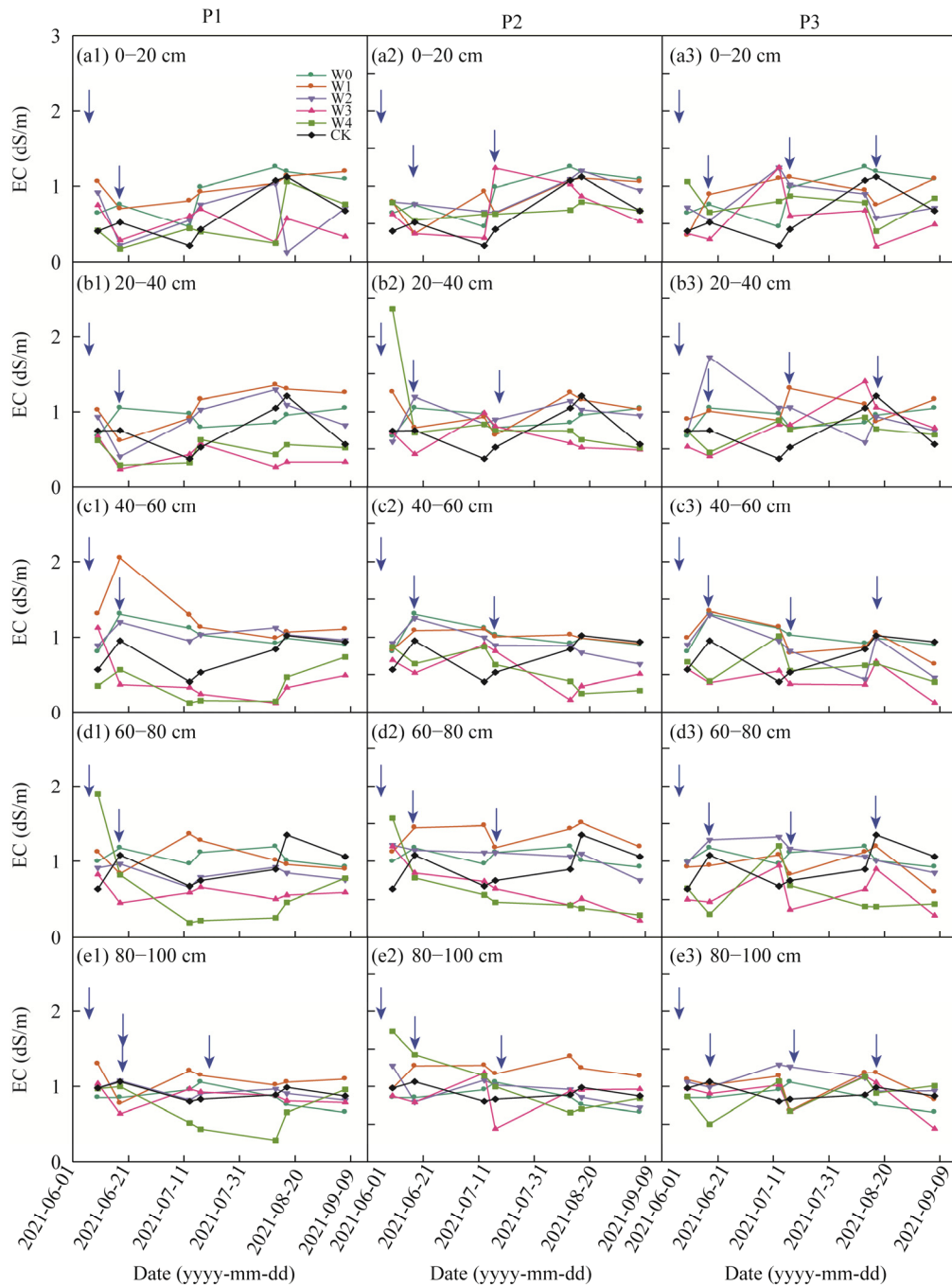
Fig. 6 Soil EC dynamics for different leaching amount and period treatments in 2021. (a1–a3), 0–20 cm; (b1–b3), 20–40 cm; (c1–c3), 40–60 cm; (d1–d3), 60–80 cm; (e1–e3), 80–100 cm. Arrow means the leaching date.
