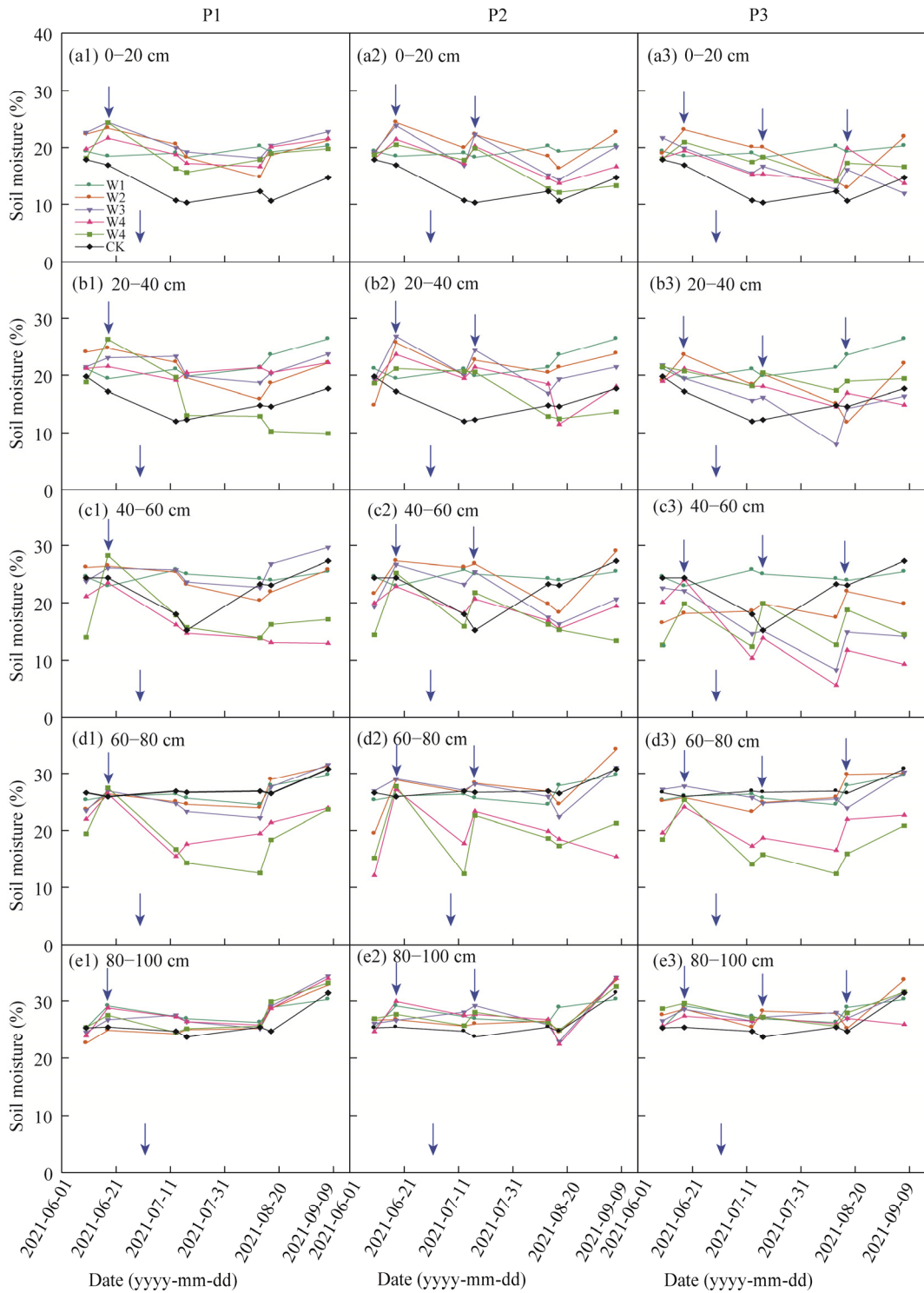
Fig. 4 Soil moisture dynamics for different leaching amount and period treatments in 2021. (a1–a3), 0–20 cm; (b1–b3), 20–40 cm; (c1–c3), 40–60 cm; (d1–d3), 60–80 cm; (e1–e3), 80–100 cm. Arrow means the leaching date.
