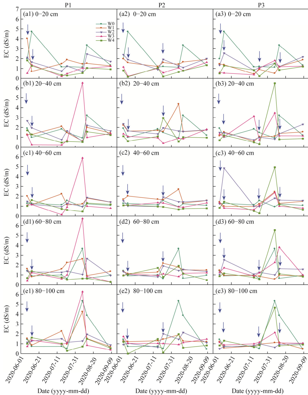
Fig. 5 Soil electrical conductivity (EC) dynamics for different leaching amount and period treatments in 2020. (a1–a3), 0–20 cm; (b1–b3), 20–40 cm; (c1–c3), 40–60 cm; (d1–d3), 60–80 cm; (e1–e3), 80–100 cm. Arrow means the leaching date.
